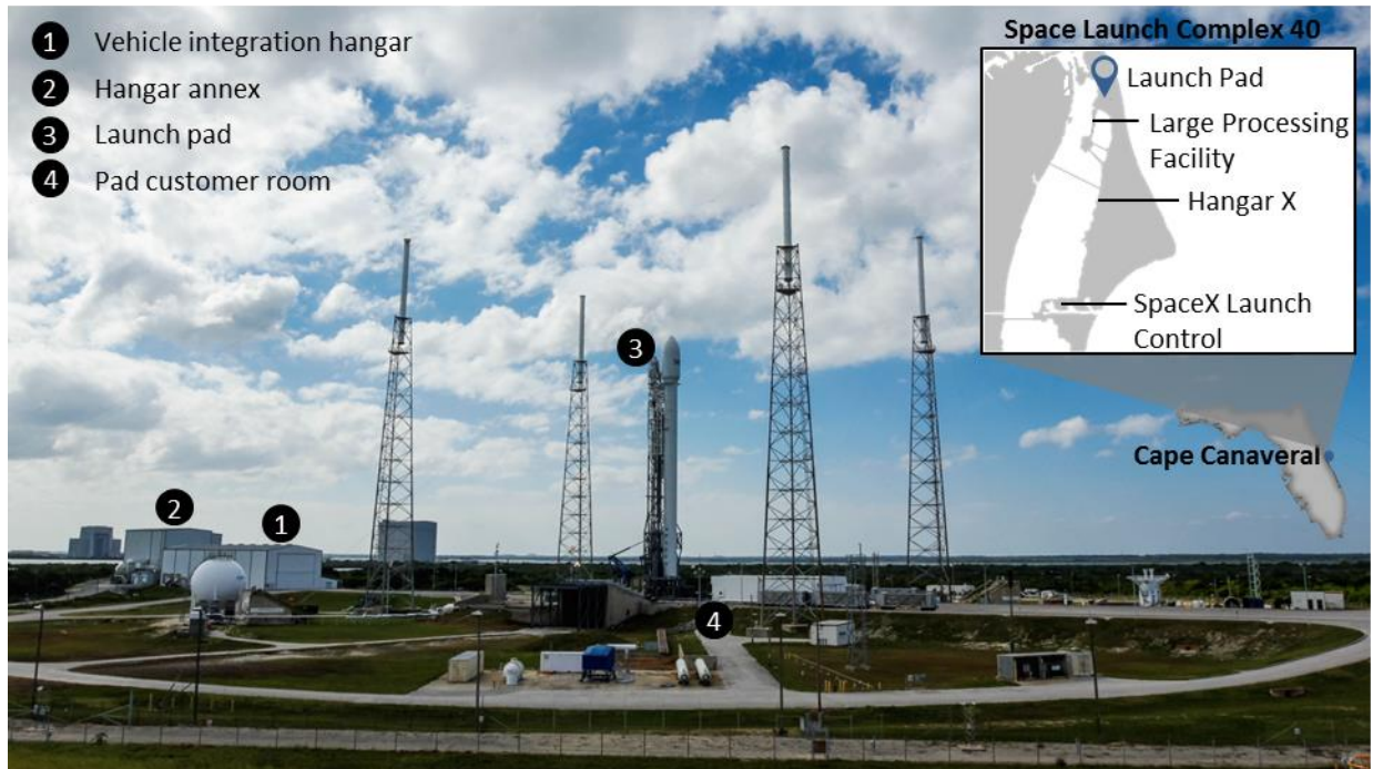
Figure 6-1: Space Launch Complex 40 at Cape Canaveral Space Force Station, Florida
